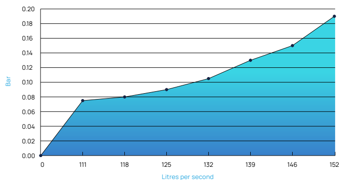
DN250 (10") PRESSURE DROP GRAPH
